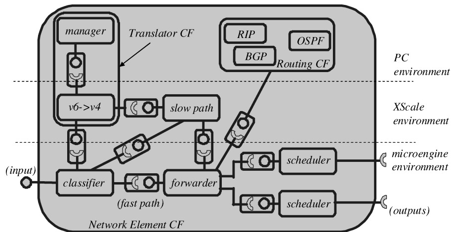
Fig. 6. Outline of an Intel IXP-based router.
