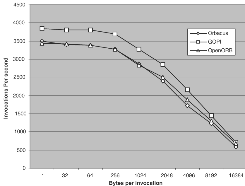
Fig. 8. Performance of OpenORB versus GOPI and Orbacus.
