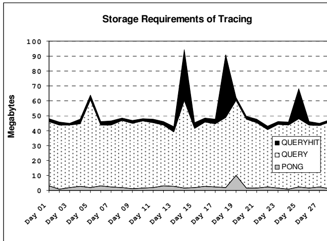
Figure 3. Storage Requirements of Tracing
